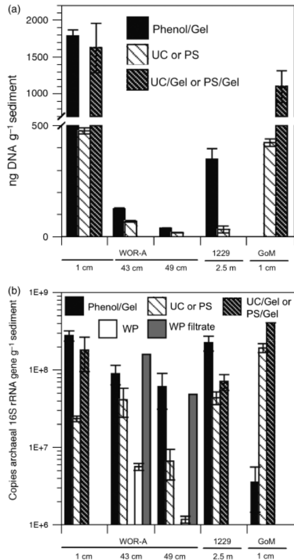
Fig. 4. Comparisons of different DNA extraction/purification methods. (a) PicoGreen-measured \text{ngDNA g}^{-1} whole sediment. Error bars for WOR-A depths 43 and 49 cm represent the average SD in the triplicate standard curve; for the PowerSoil/gel measurements, the difference between two measurements is shown; all other error bars are the SD of triplicate sample measurements. Only samples WOR-A (43 and 49 cm) underwent the phenol/WizardPlus procedure; these measurements were below 3 \text{ ng g}^{-1} sediment and are not visible on the plot. For WOR-A 49 cm and 1229, measurements of the UltraClean/gel and PowerSoil/gel groups were below the PicoGreen detection limit. WOR-A 43 cm did not undergo the UltraClean/gel procedure. (b) qPCR-determined copies of archaeal 16S rRNA genes \text{g}^{-1} whole sediment. Error bars represent the SD of triplicate sample measurements. For duplicate sample measurements, such as UltraClean/gel, PowerSoil/gel, and WOR-A 43 cm phenol/WizardPlus, the differences are shown, and phenol/WizardPlus filtrate values are from a single measurement. UC, UltraClean; PS, PowerSoil; WP, WizardPlus.
