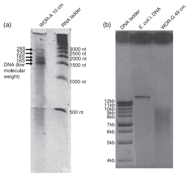
Fig. 3. (a) RNA extracted with phenol/bead-beating, RNeasy, and acrylamide gel clean-up showing intact RNA subunits next to the RNA Millenium Markers (Ambion), stained with SYBR Gold on a denaturing gel with 20% acrylamide overlying 80% acrylamide (transition visible near 500 nucleotides). (b) DNA extracted with phenol/bead-beating and acrylamide gel clean-up showing degraded DNA next to genomic DNA from lambda Escherichia coli and a 1-kb DNA ladder (Invitrogen). Sample was from July 2008 core G, and was stained with ethidium bromide and run on a nondenaturing 1.5% agarose gel. Lanes were digitally cut from a single gel picture and moved next to each other to avoid lanes from another experiment.
