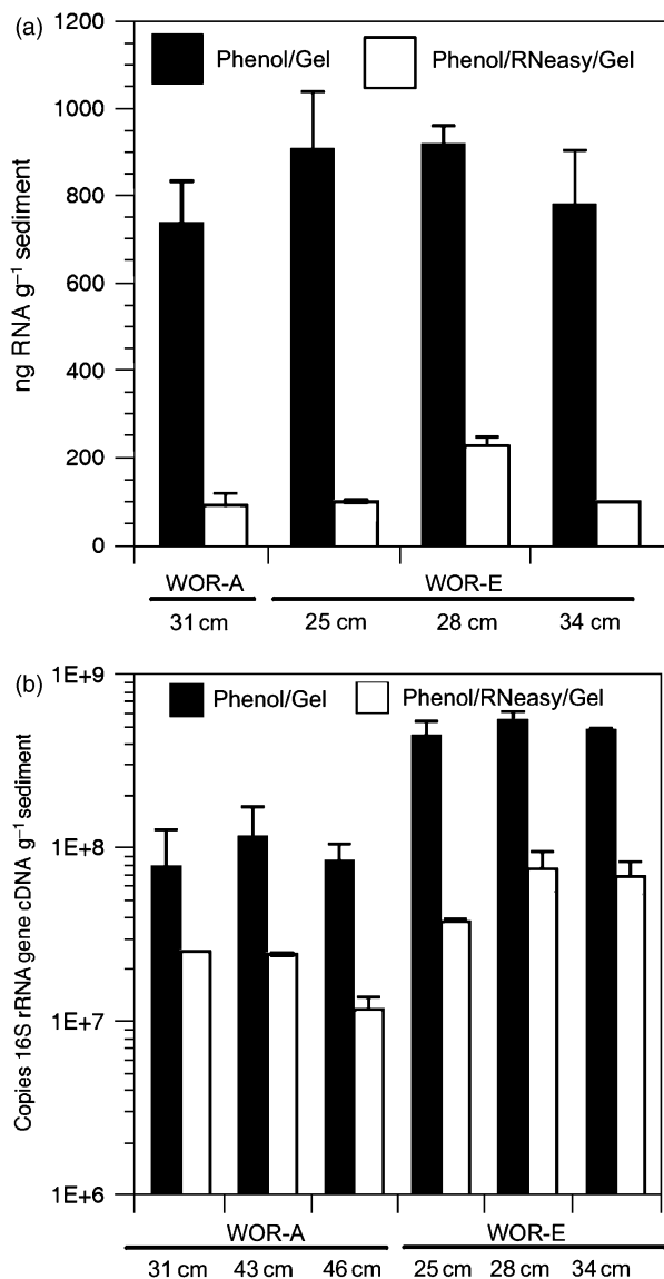
Fig. 2. Comparisons of RNA yield using different RNA purification methods listed in Fig. 1. RNA recovery from sediment samples from WOR cores A and E; depths below sediment surface are given for individual subsamples within each core. (a) RiboGreen quantification of ngRNA g -1 whole sediment. All error bars represent the SD of triplicate sample measurements, except WOR-E 28 cm phenol/gel, where the difference between duplicate measurements is shown. (b) RT-qPCR of archaeal 16S rRNA cDNA g -1 whole sediment. Error bars for phenol/gel values represent the SD of triplicate sample measurements; for phenol/RNeasy/gel results, the difference between duplicate measurements is shown. The phenol/RNeasy/gel result for sample WOR-A 31 cm is a single measurement.
