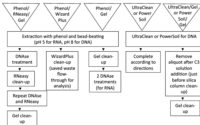
Fig. 1. Flowchart of each extraction/purification procedure, with the names of each procedure in the header arrows. UC, Ultra Clean; PS, PowerSoil; WP, WizardPlus.
